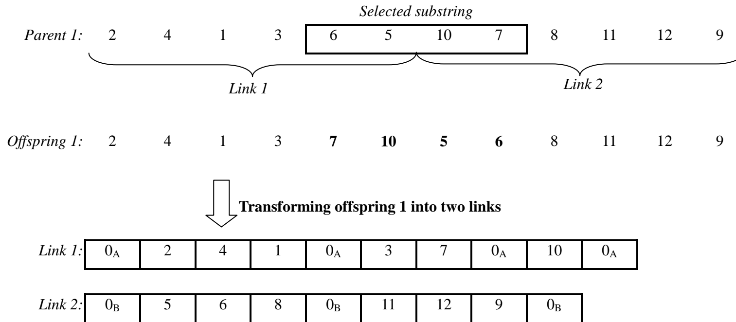
Fig. 8. The inversion mutation operator.
